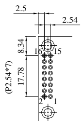
PIN DETAIL
