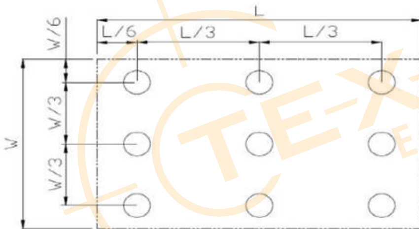
Fig 5.3. Definition of uniformity
