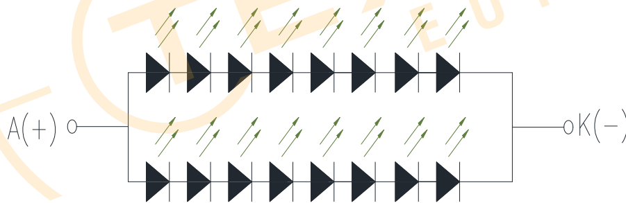
B/L Circuit
