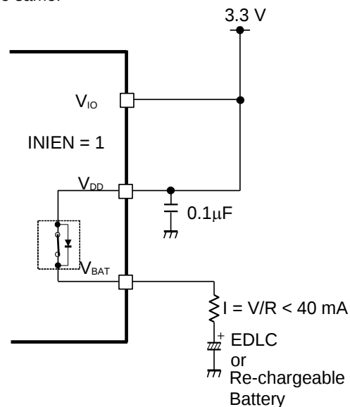
Figure 5 Circuit Ex.2
