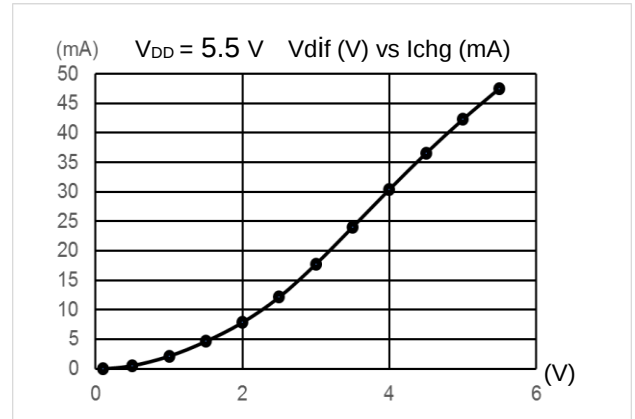
Figure 11 Chargeable Current of VBAT ( V_{DD} = 5.5\text{ V} )
