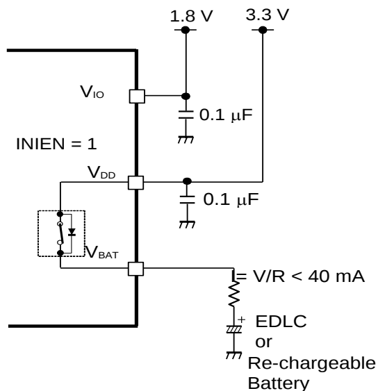
Figure 4 Circuit Ex.1
