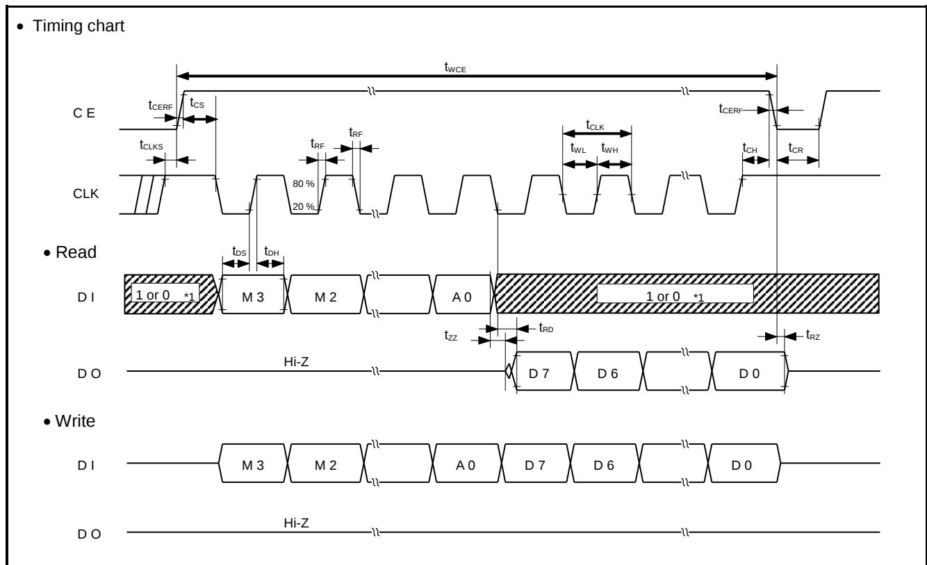
Figure 13 SPI-Bus Timing Chart
