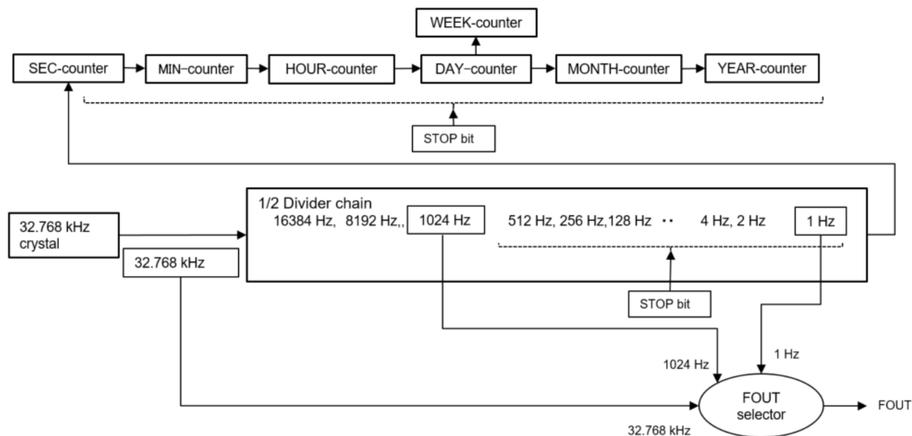
Figure 19 Basic Function 32.768 kHz oscillation, counter, FOUT
