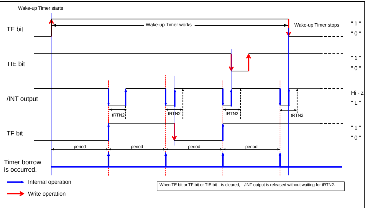
Figure 24 Wake-up Timer Timing Chart
