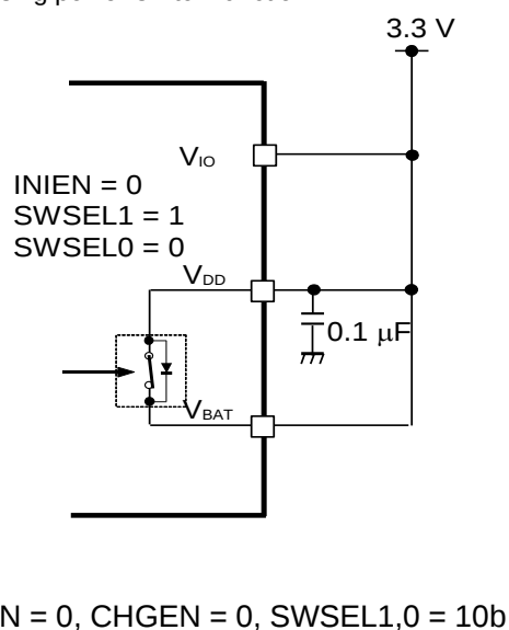
Ex.4 Not using power-switch function
