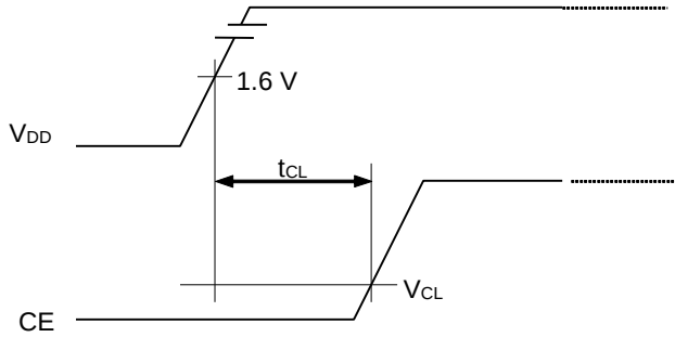
Figure 15 VDD, CE sequence
