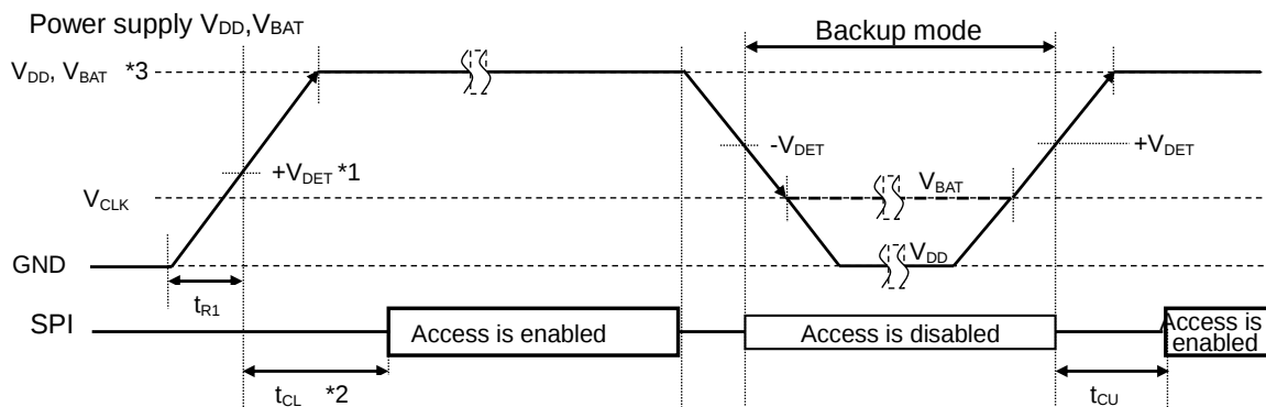
Figure 14 Power on Sequence
