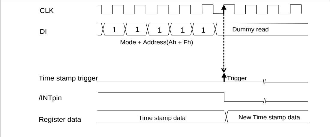
Figure 35 Time Stamp SPI-Bus record timing
