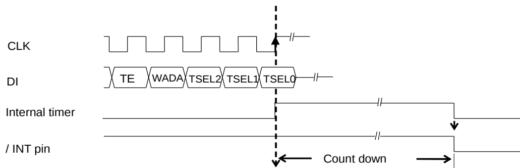
Figure 22 Wake-up Timer Start Sequence
