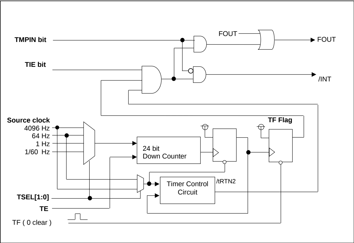
Figure 23 Wake-up Timer Block Diagram
