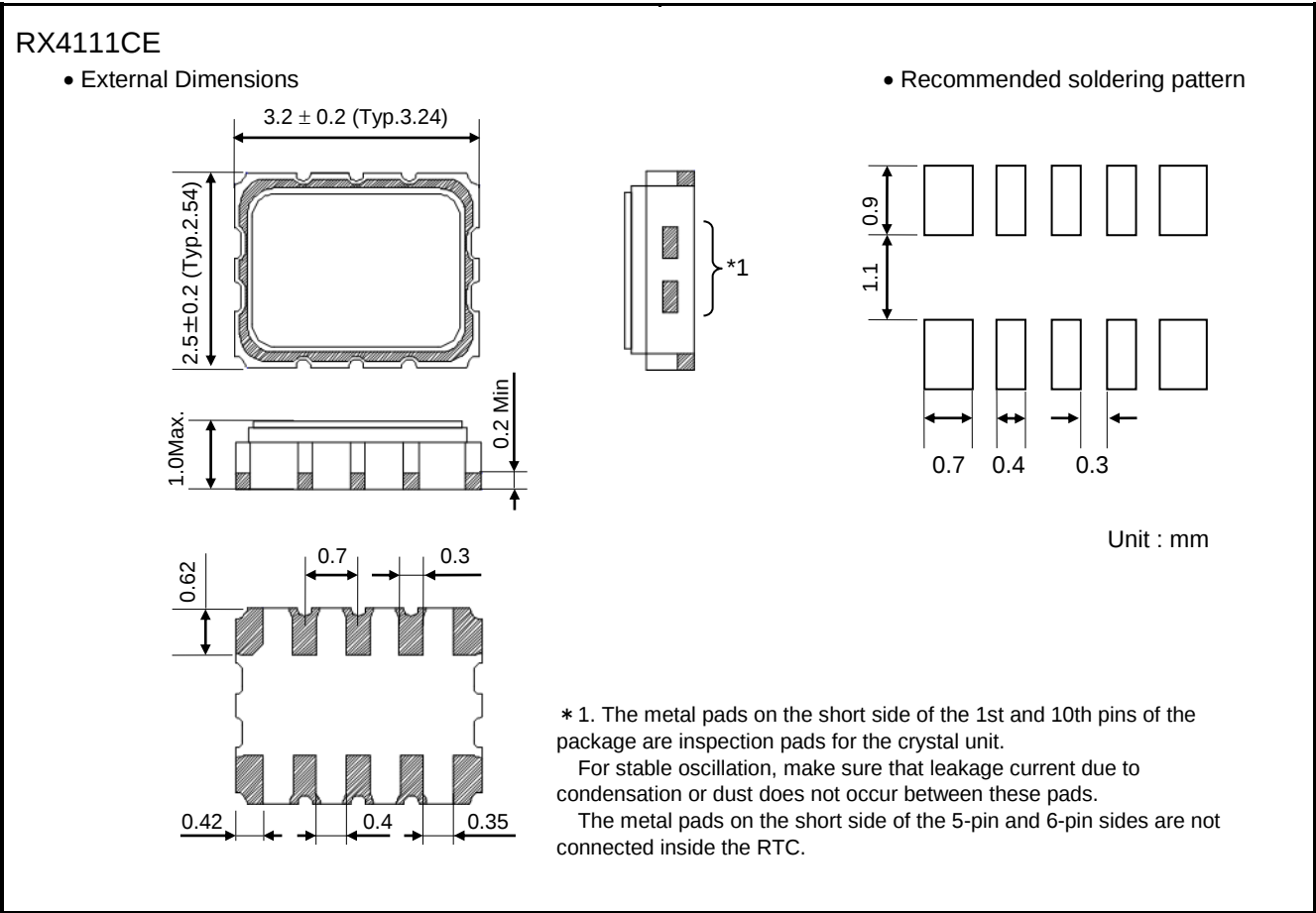
Figure 8 External dimensions
