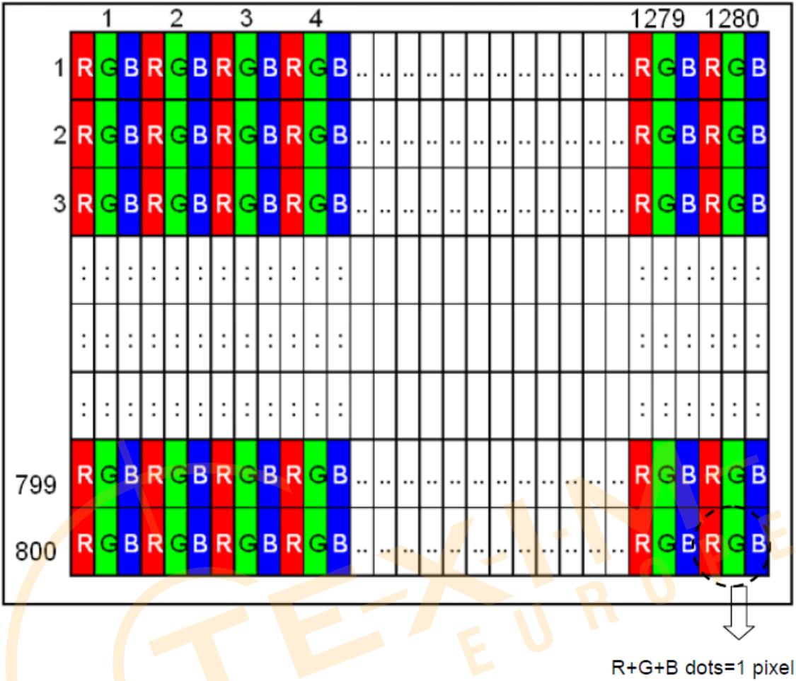
Figure 2 Pixel Format
