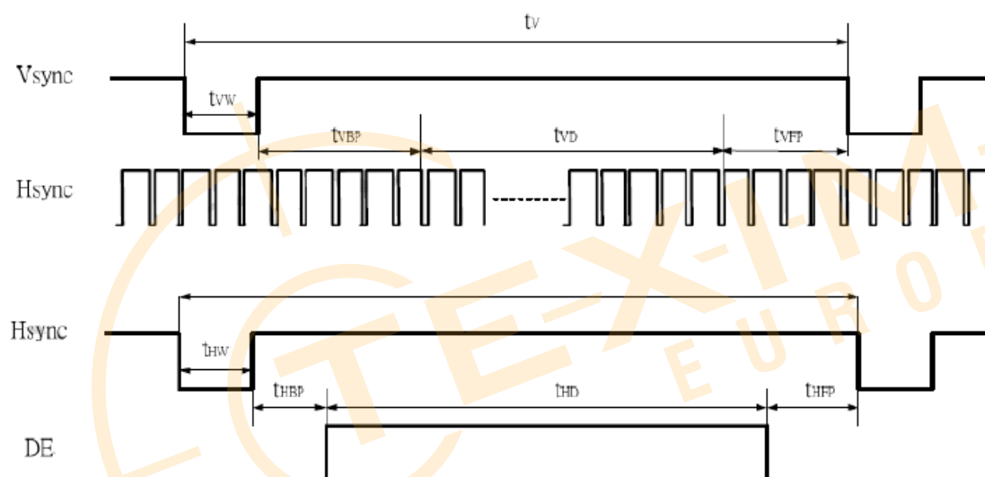
Figure 8 Timing Characteristics
