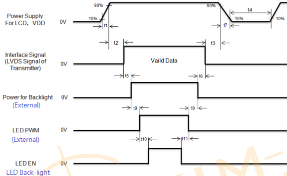
Figure 12 Power Sequence
