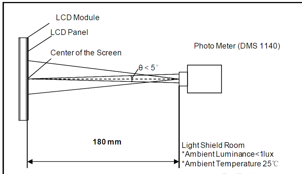
Figure 4 Measurement Setup
