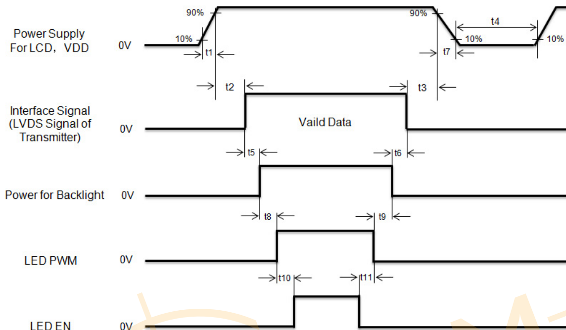
Figure 12 Power Sequence
