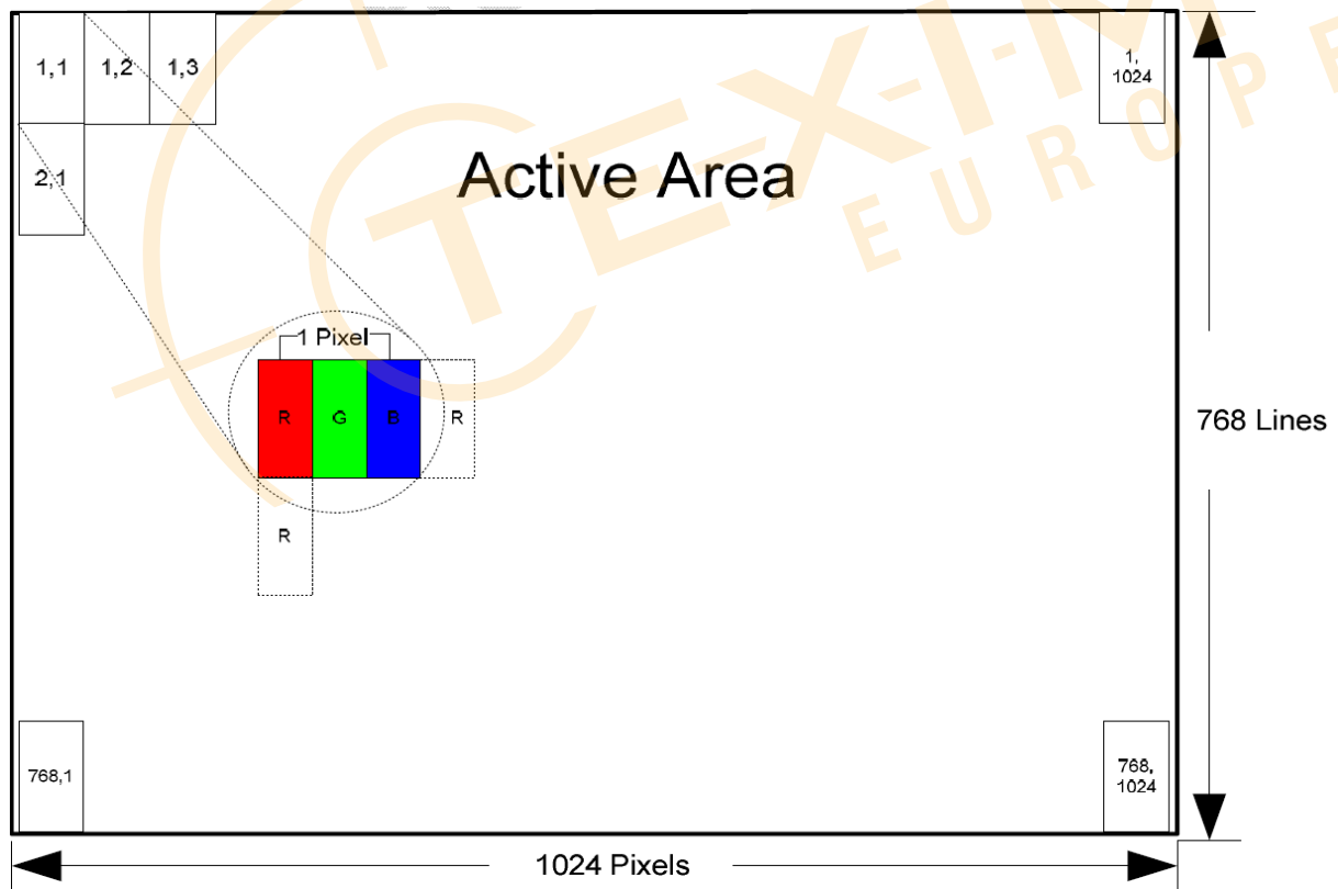
Figure 2 Pixel Mapping
