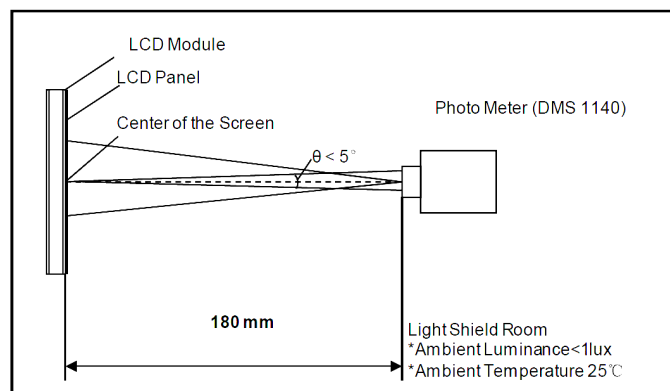
Figure 4 Measurement Setup
