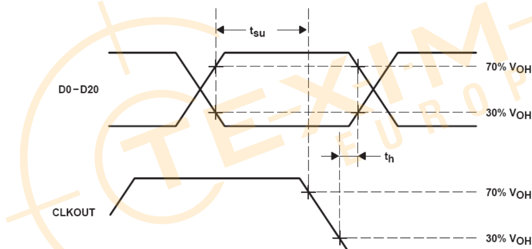
Figure 5. Setup and Hold Time Waveforms
