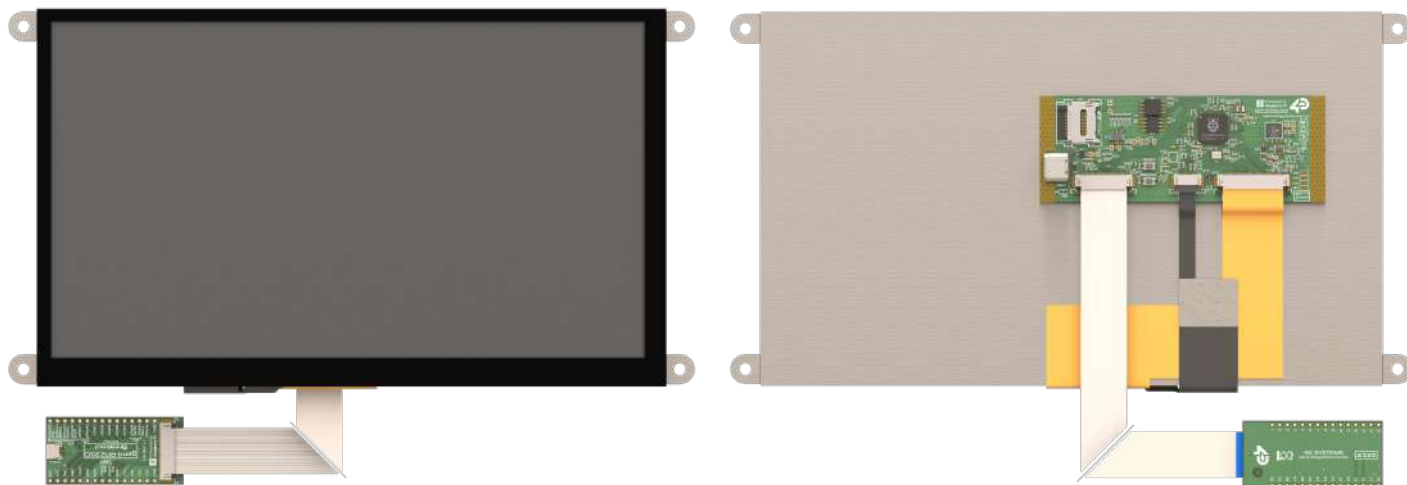
gen4-RP2350 Breakout Front
