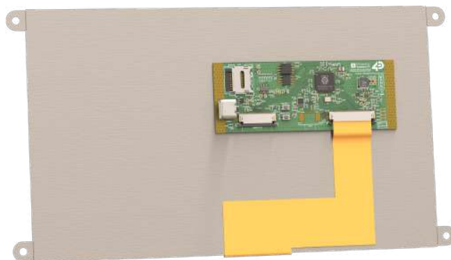
RP2350-90T Rear
