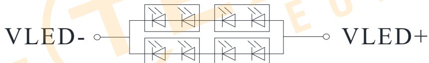
Backlight Circuit
