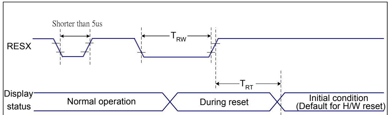
Figure 7 Reset Timing
