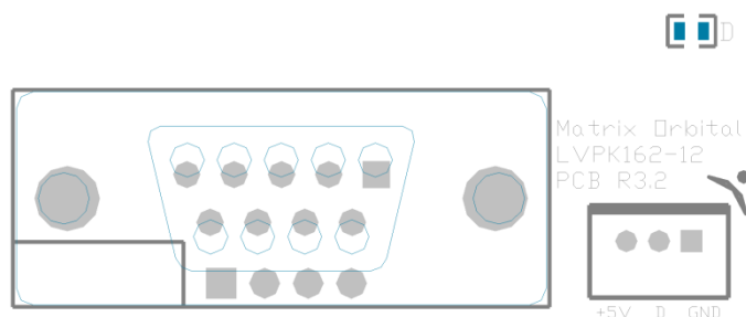
Figure 10: Power Through DB9 Jumper
