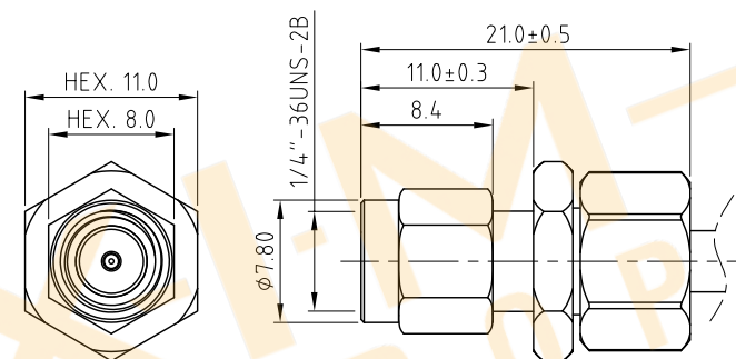
SMA PLUG DETAIL DRAWING
