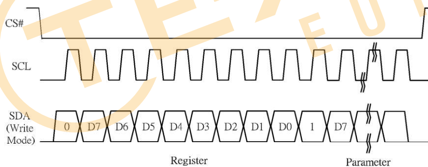
Figure 6-3: Write procedure in 3-wire SPI mode
