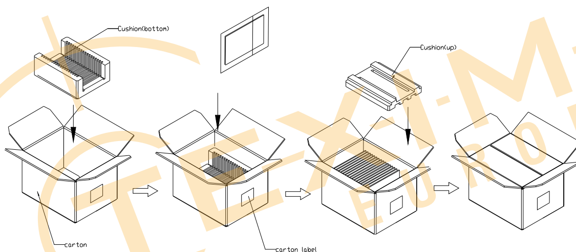
Figure. 9-1 Packing method
