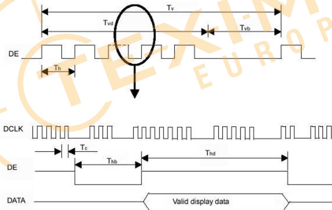
INPUT SIGNAL TIMING DIAGRAM
