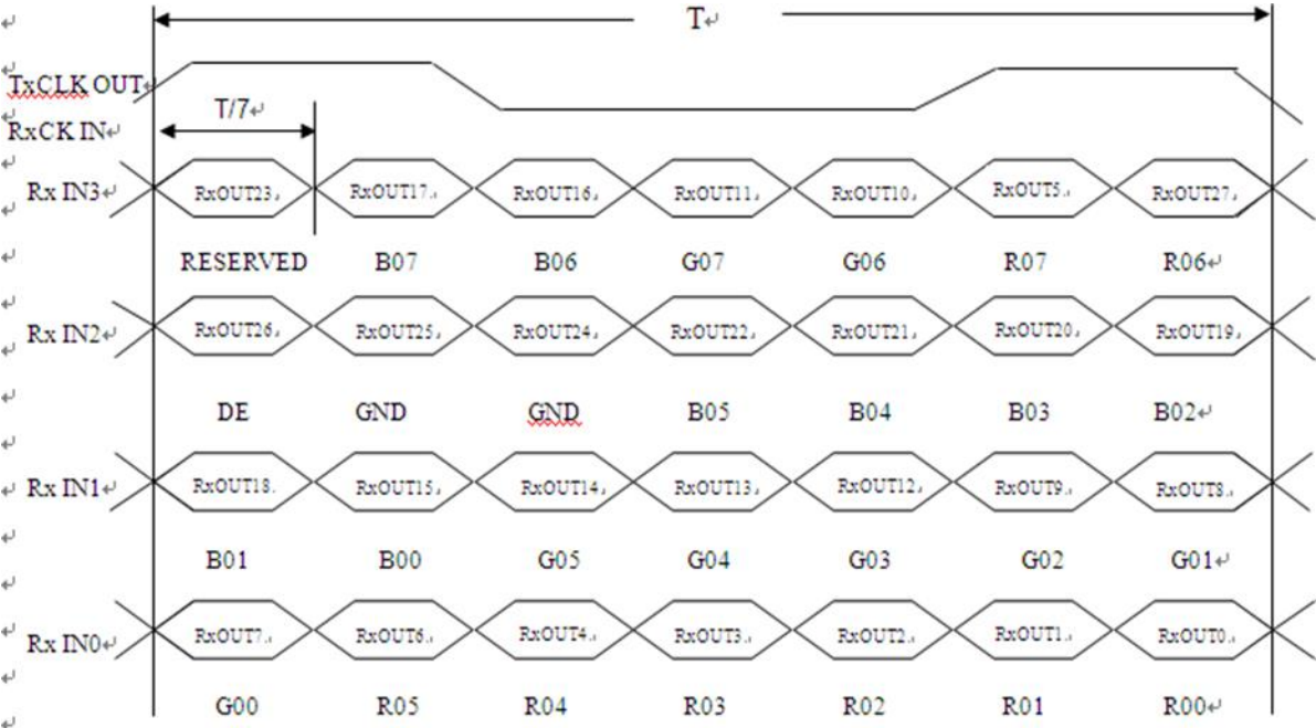
INPUT SIGNAL TIMING DIAGRAM TIMING DIAGRAM of LVDS
