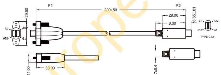
Dual-side Lockable USB-C Cable P/N : 9480240240K6
