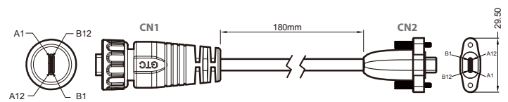
Waterproof USB-C to Lockable USB-C Cable P/N : 9480240240K8
