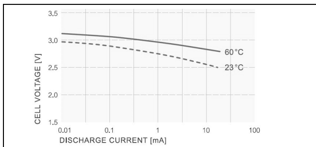
*Discharge depth 50%
