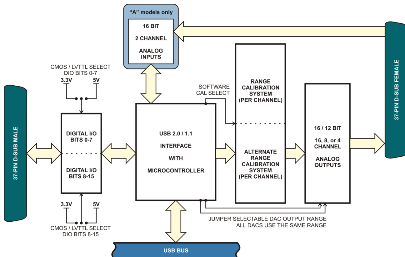
Figure 1-1: Block Diagram
