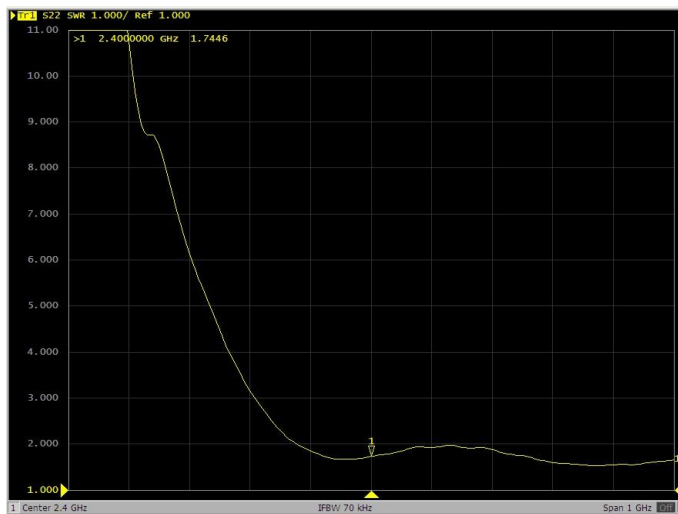
VSWR at 2.4GHz
