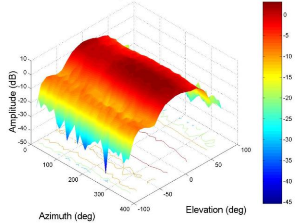
Plane radiation at 2.4GHz.jpg
