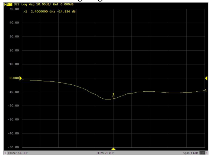
Log Mag at 2.4GHz
