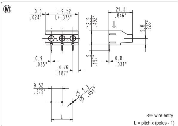
MSP_09N-000E 90°, low ampere rating, modular
