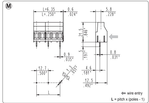
MSP_00U straight, modular
