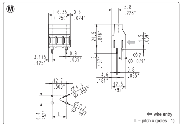
MSP_00U-0000P straight, modular with VDE pegs
