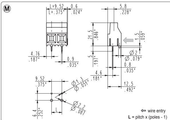
MSP_00N-0000P straight, modular with VDE pegs
