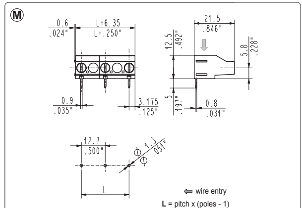
MSP_09U-000E 90°, low ampere rating, modular
