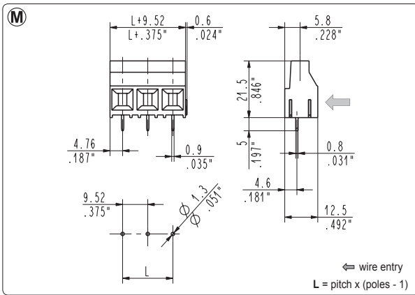
MSP_00N straight, modular
