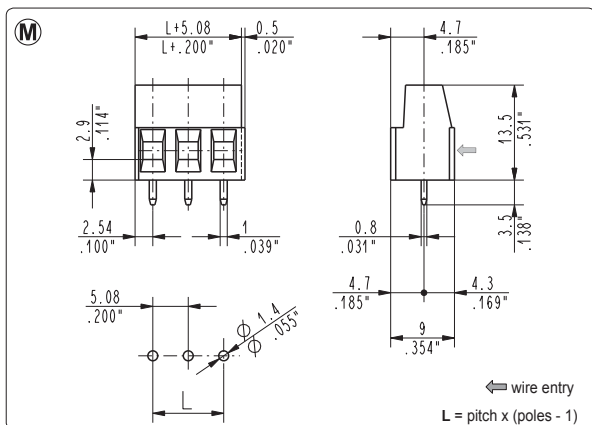
MSG_005-000C straight, modular, short circuited
