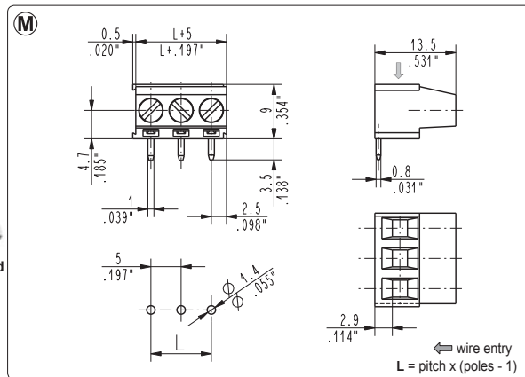
MSG_091-000C 90°, modular, short circuited
