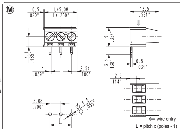
MSG_095-000C 90°, modular, short circuited
