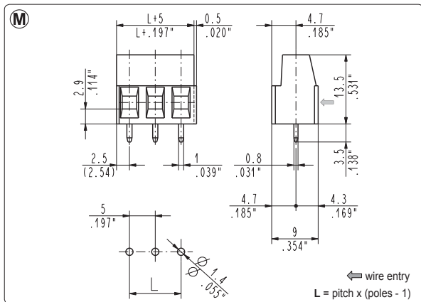
MSG_001-000C straight, modular, short circuited
