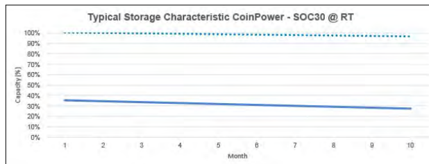
Storage Characteristic @ Various Temperatures Remaining Capacity
