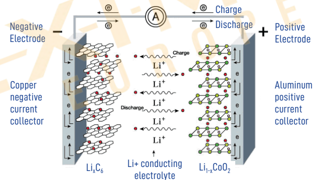
Chemical reaction in Li-Ion rechargeable battery
