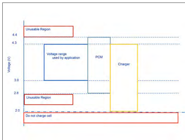
Voltage range for PCM and Charger for CoinPower A4 series
