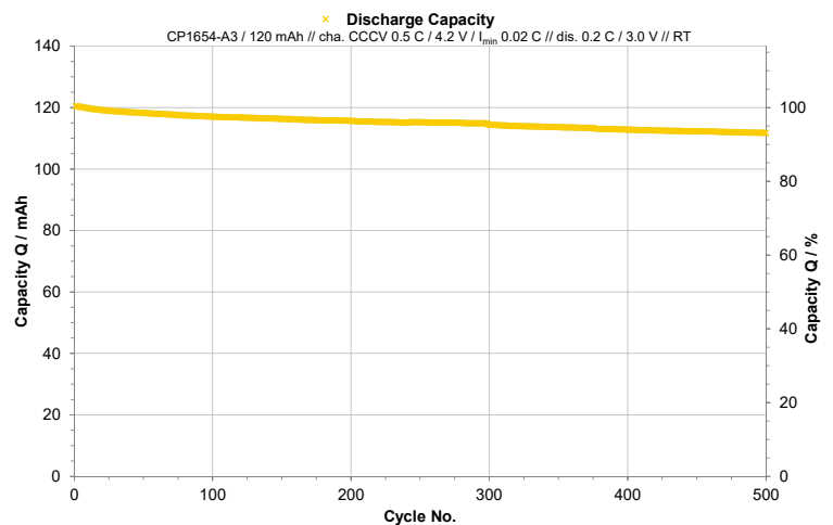
CoinPower CP1654 A3 Discharge Performance – 0.5C/0.2C
