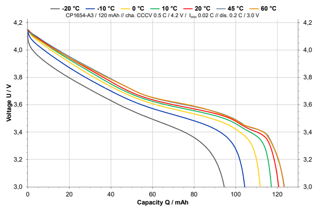
CP1654 A3 – Discharge Characteristic at various temperatures
