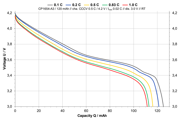
CP1654 A3 – Discharge Characteristic with different loads
