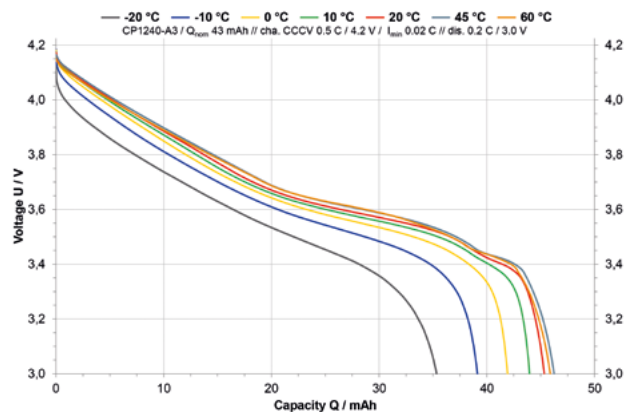
CP1240 A3 – Discharge Characteristic at various temperature
