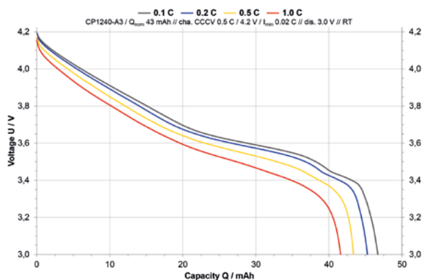
CP1240 A3 – Discharge Characteristic with different loads
