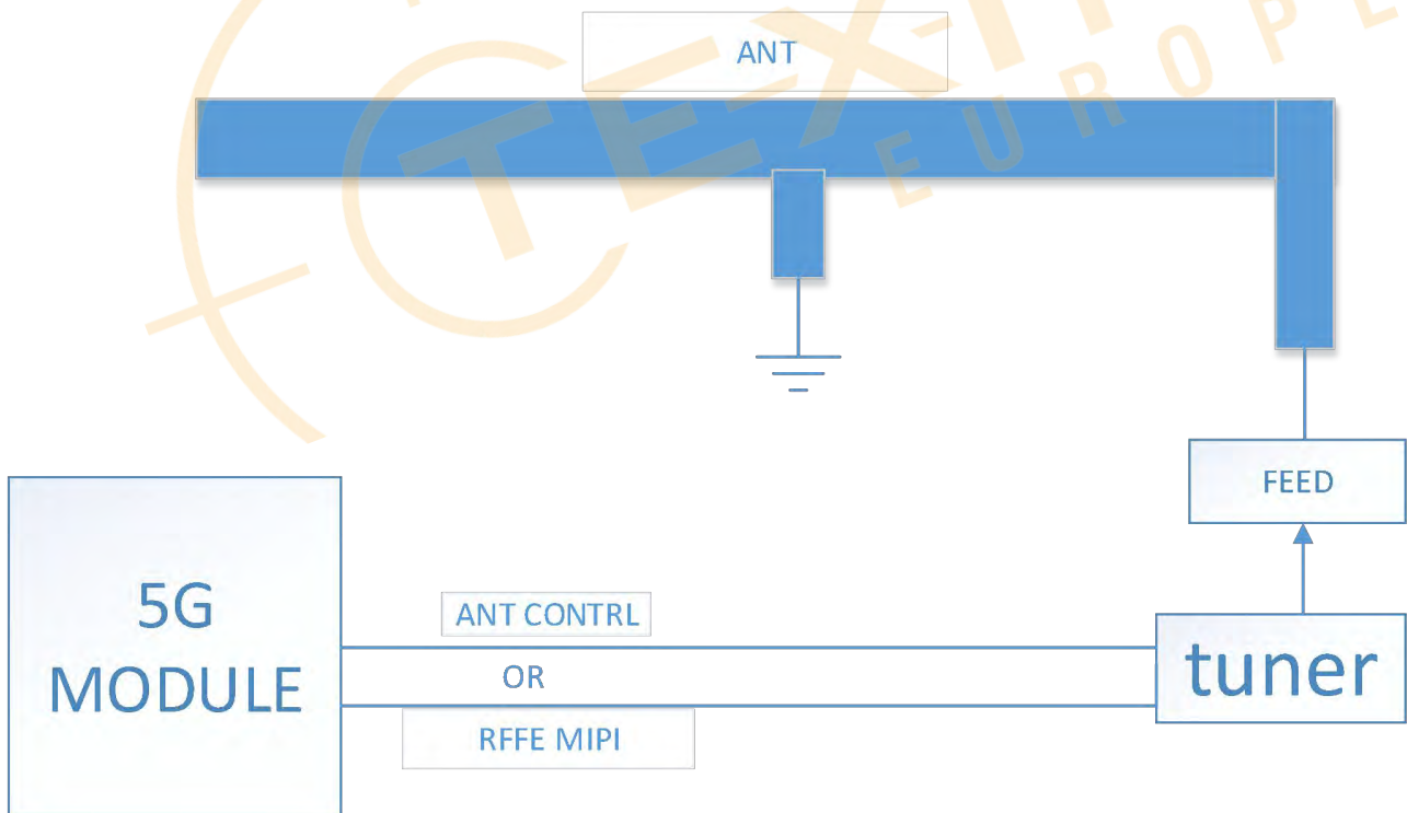
Figure 29: Impedance tuner reference block diagram
