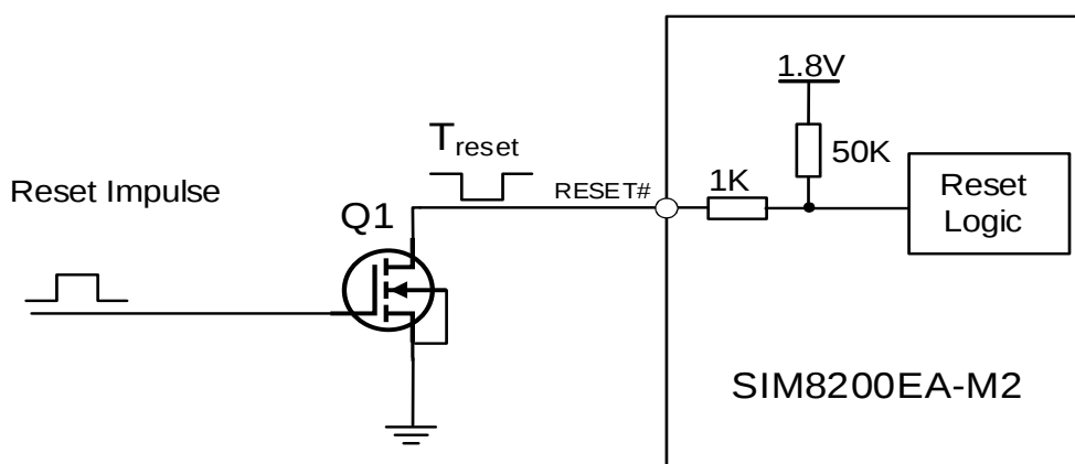
Figure 11: Reference reset circuit
