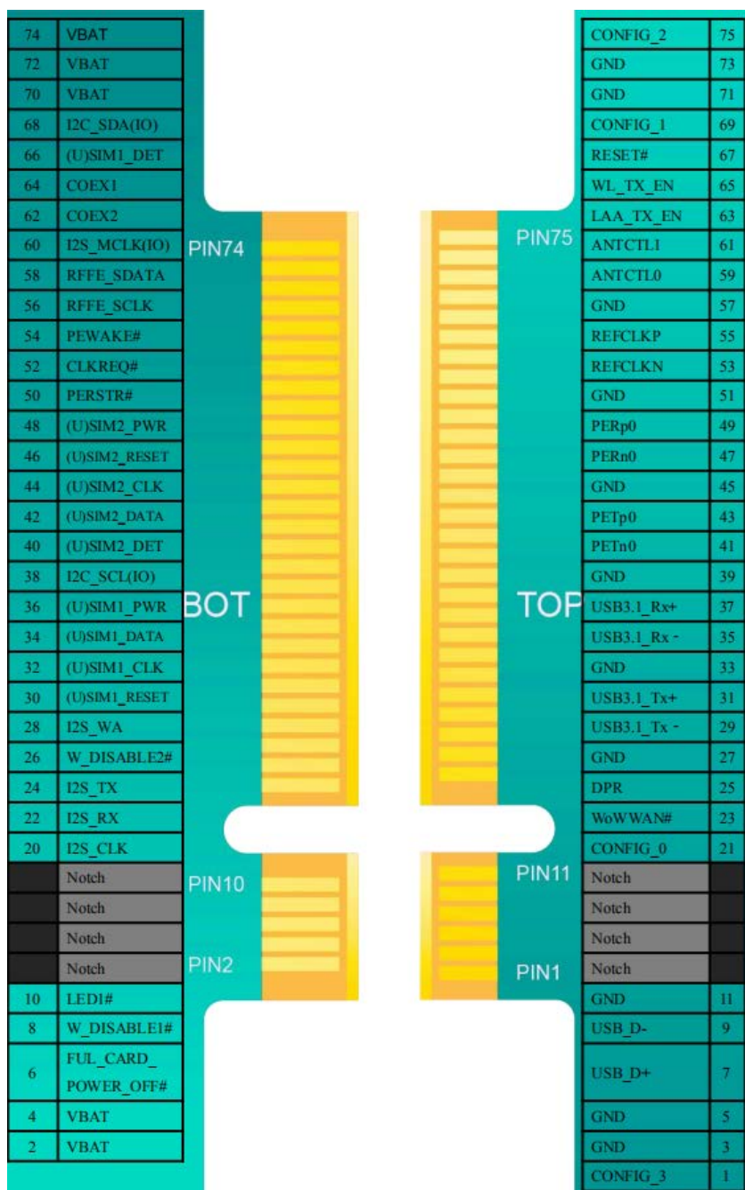
Figure 2: Pin assignment
