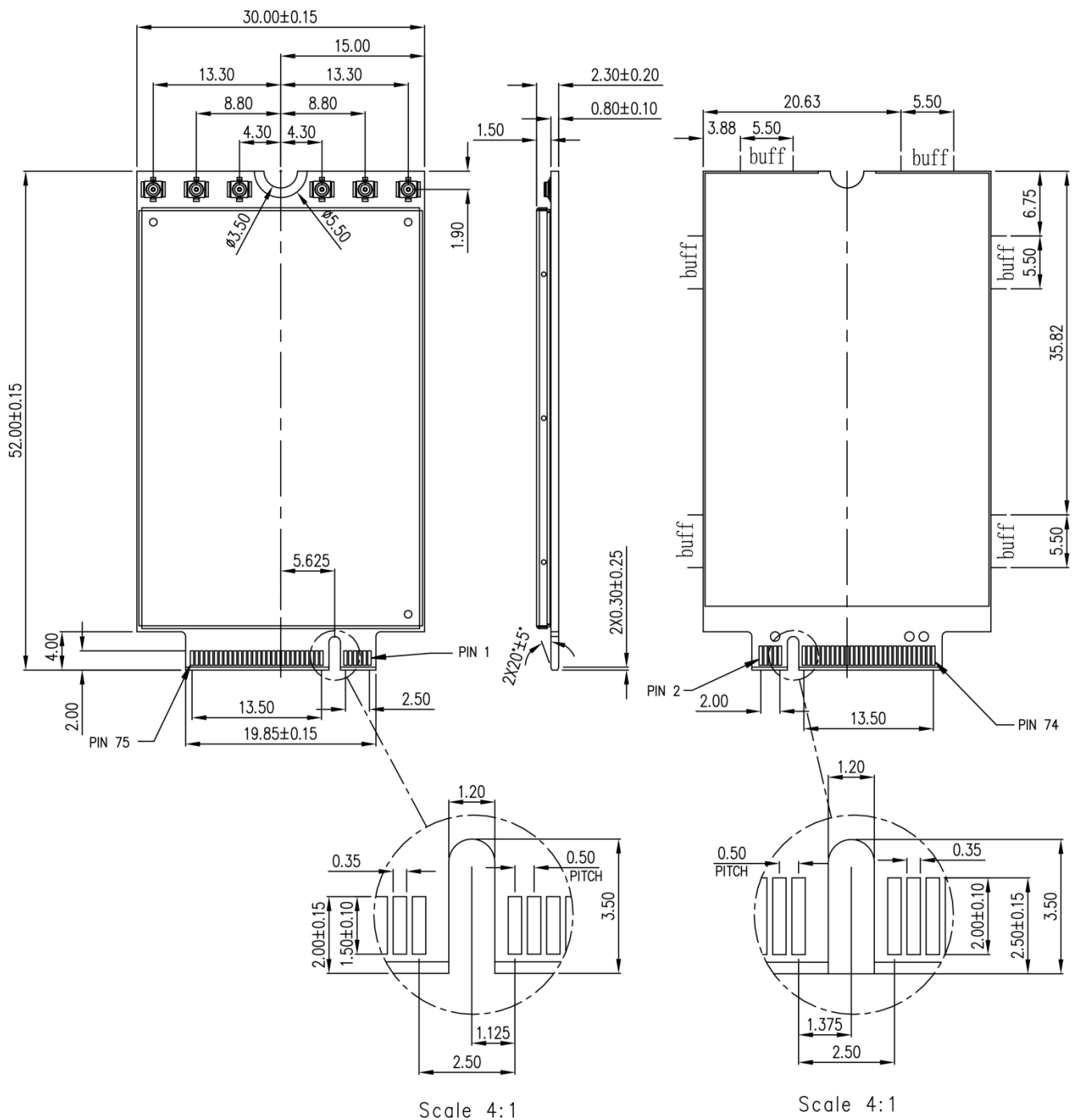
Figure 3: Dimensions of the module (unit: mm)
