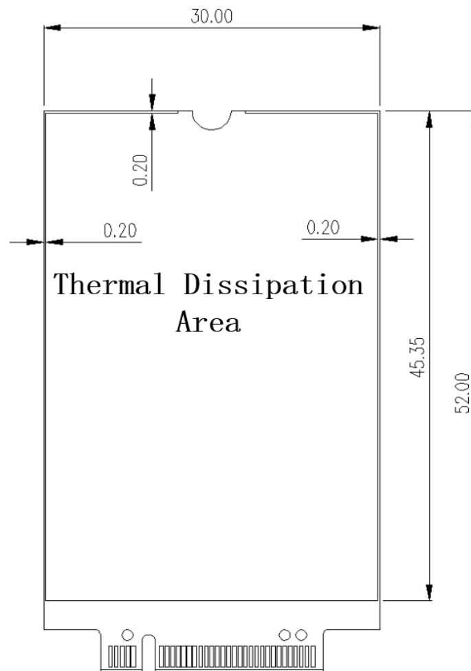
Figure 27: Thermal dissipation area on bottom side of the module
