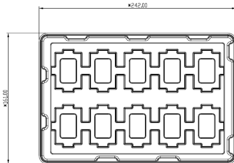
Figure 30: Packaging procedures
