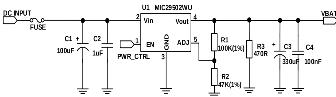
Figure 6: Linear regulator reference circuit
