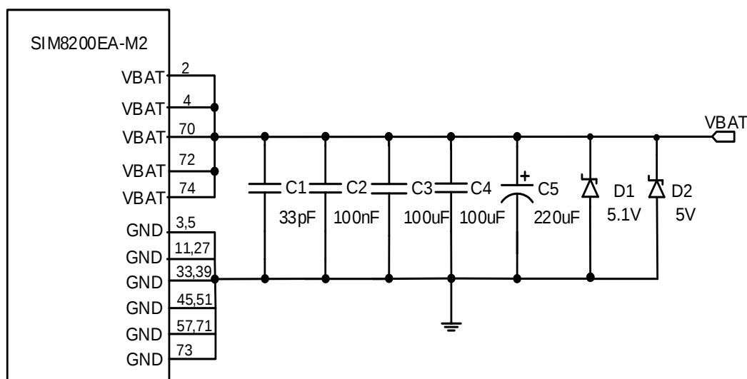
Figure 5: Power supply application circuit
