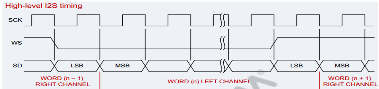
Figure 19: I2S timing
