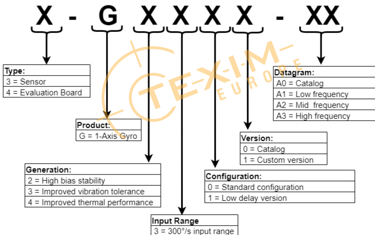
Figure 28: Ordering information
