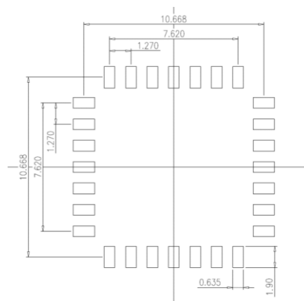
Figure 15: Recommended Pad Layout in mm (top view)
