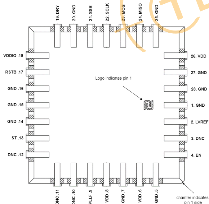
Figure 13: GYPRO4300 Sensors Pinout (bottom view)
