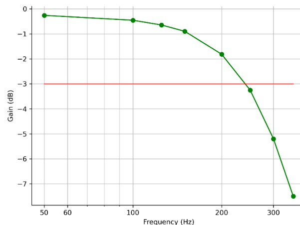
Figure 10: Frequency response (room temperature)
