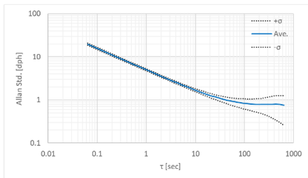
Figure 3.1 Gyro Allan Variance Characteristic (M-G366PDG0)
