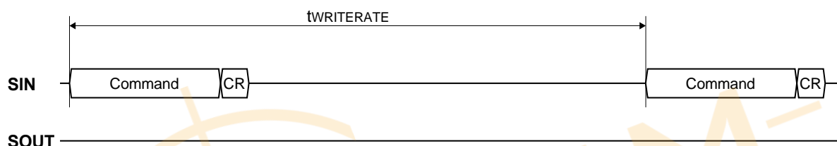
Figure 5.7 UART Write Timing
