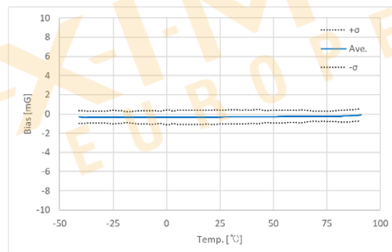
Figure 3.11 Accelerometer Bias vs. Temperature Characteristic (M-G330PDG0)
