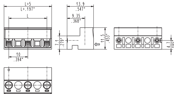
⇐ wire entry L = pitch x (poles - 1)
