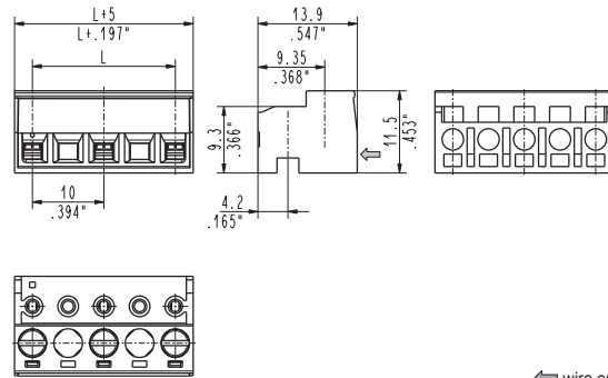
⇐ wire entry L = pitch x (poles - 1)
