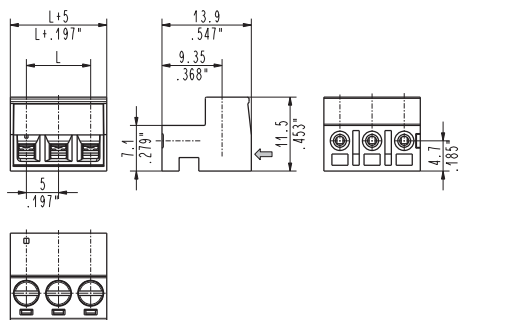
⇐ wire entry L = pitch x (poles - 1)
