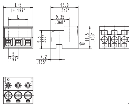
⇐ wire entry L = pitch x (poles - 1)
